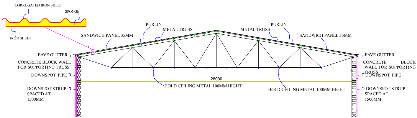
TRUSS CROSS SECTION
